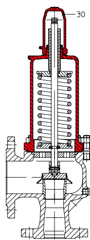
Fig. ... .911 gastight cap, closed bonnet
