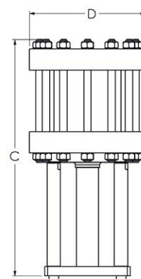
Piston Actuator Pillar Yoke
