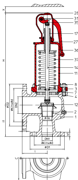
Fig. ... .901 closed lifting device, closed bonnet
