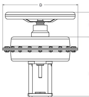
Diaphragm Actuator Pillar Yoke
